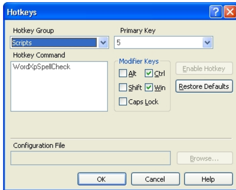
The Hotkeys dialogue
